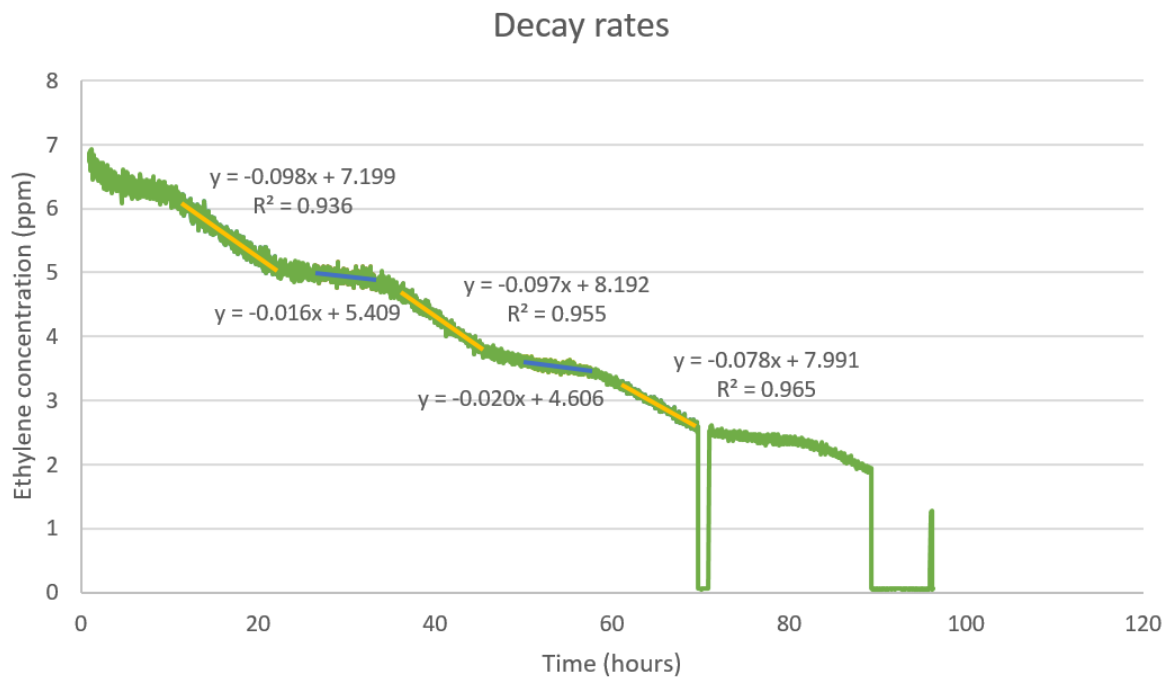
Figure 3: Decay rates determined for when the air cleaner is on (yellow) or off (blue)
